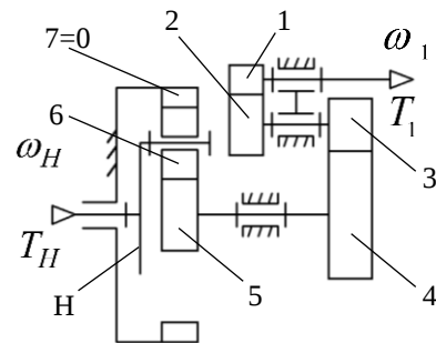
a. Structural scheme for Suzuki multiplier
