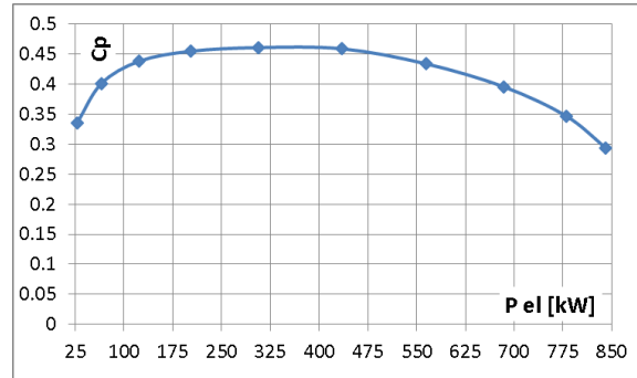
b. The efficiency depending by the electric power
