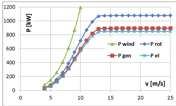
Fig. 2. The power curves for the studied wind system
