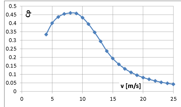
a. The efficiency depending by the wind speed
