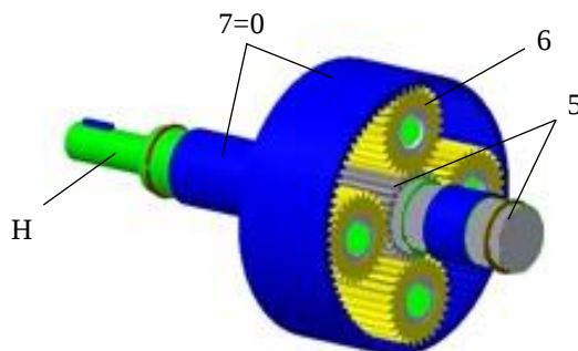
Fig.7. Planetary unit constructive variant
