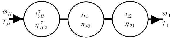
Fig.6. The speed amplifier block diagram
