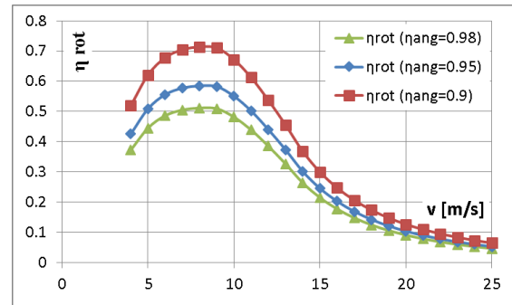
Fig. 4. The winding rotor efficiency, depending by various fixed axle gear efficiency values
