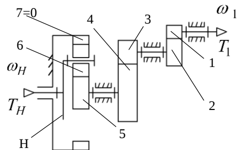
b. Structural scheme for Leimann multiplier
