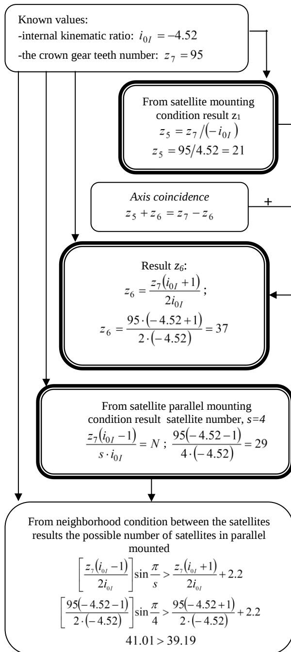
Fig.6. Teeth numbers synthesis algorithm
